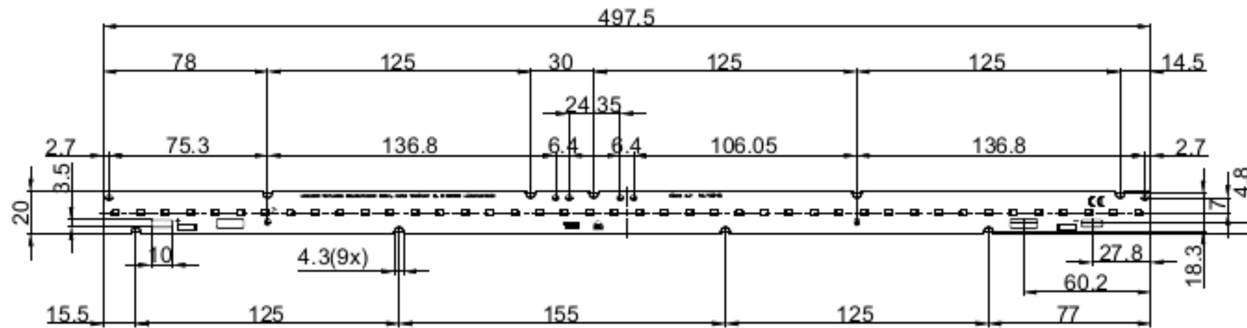
WU-M-673-STC
