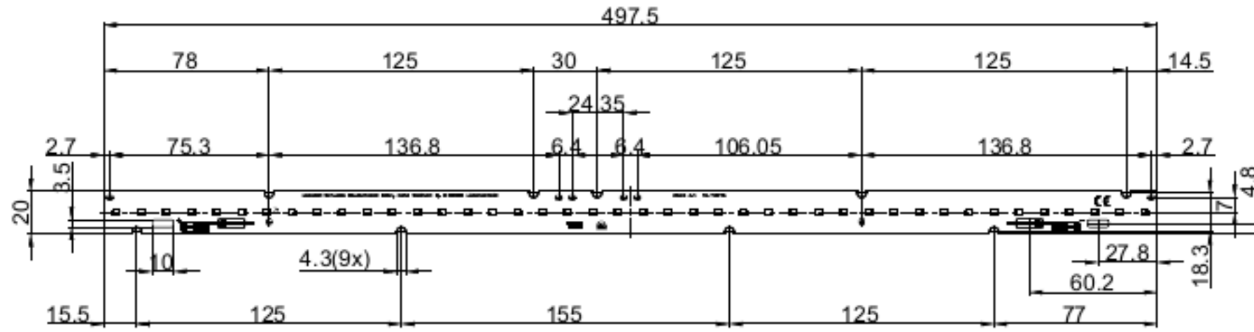
WU-M-673-BC/TC
